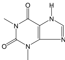
2. Theophylline
