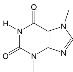
1. Theobromine
